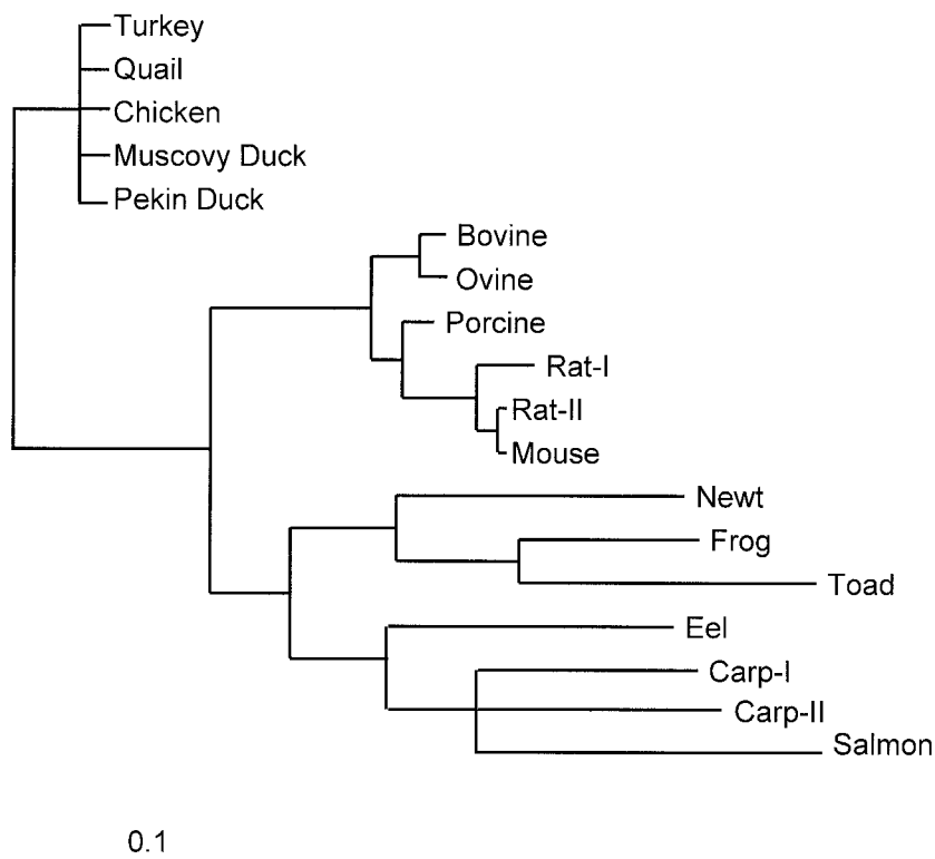
FIGURE 4 A phylogenetic tree of amino acid sequences of selected vertebrate PGH \alpha subunits. The tree was constructed with the ClustalW program by pair-group cluster method (EMBL-European Bioinformatics Institute) and Tree View (Rod Page, University of Glasgow, UK) based on available data in birds and amphibians, and selected species of mammals and teleosts as described in Fig. 2. No data are yet available for reptilian PGH \alpha . The value indicated is the number of substitutions per site.
